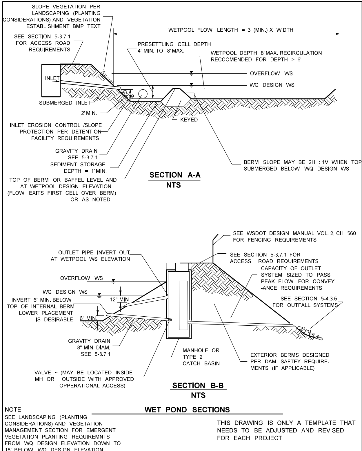
Figure 5-32 Wet pond: Cross section.
