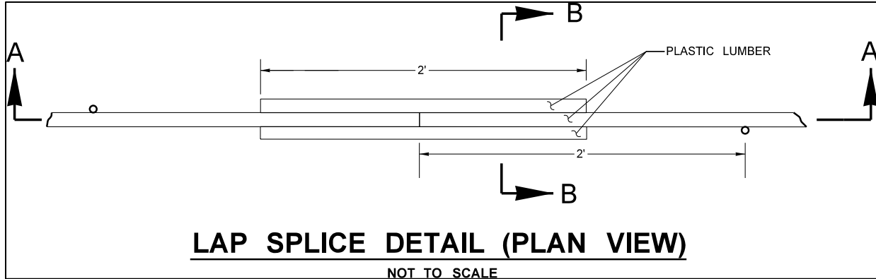
Figure 5-15 Biofiltration swale: Divider splice details.
