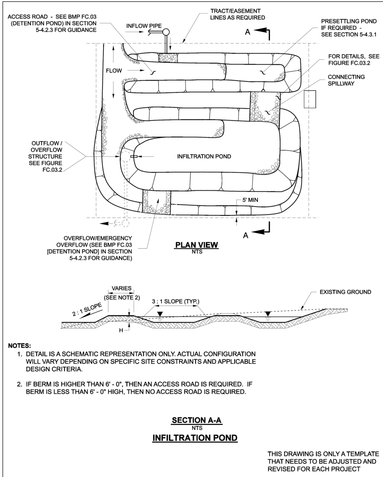
Figure 5-41 Infiltration pond.
