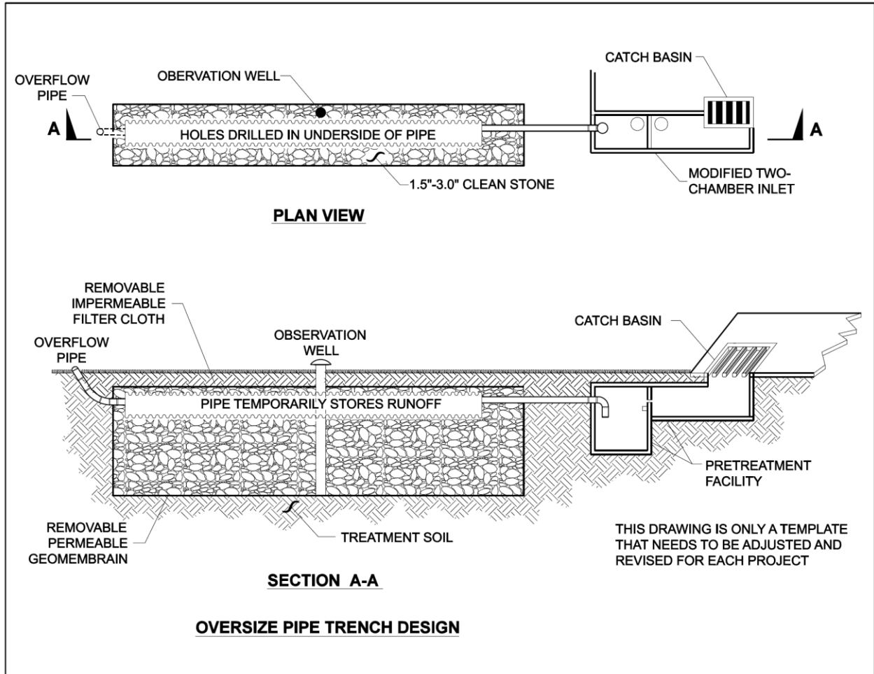
Figure 5-45 Oversize pipe trench design.
